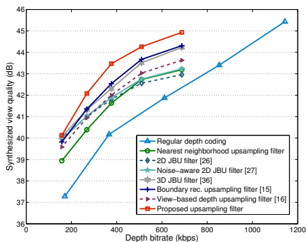
Fig. 10. RD curves obtained by reconstructing the decoded depth video using different upsampling filters and the regular depth coding at the original resolution for the Undo-Dancer sequence.
